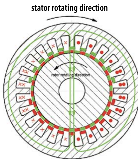
EMF Motor® lift motor principle
