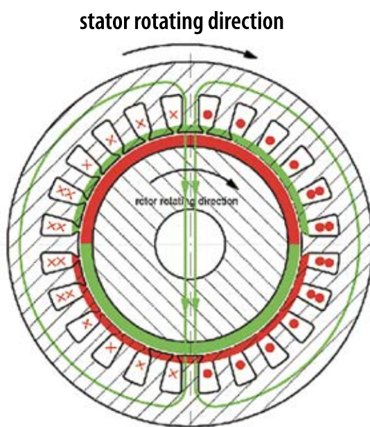
Standart lift motor principle
